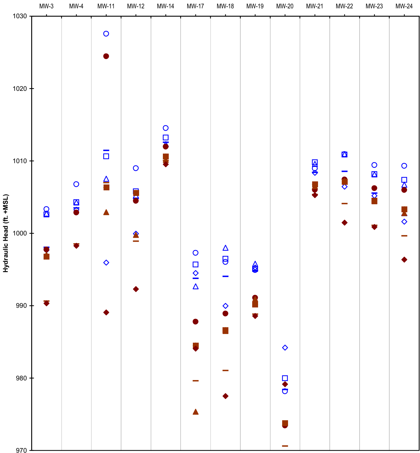
FIGURE 5-3 Hydraulic Head Elevations From Deep Multi-Port Wells July-August 2004 Jet Propulsion Laboratory Pasadena, California
